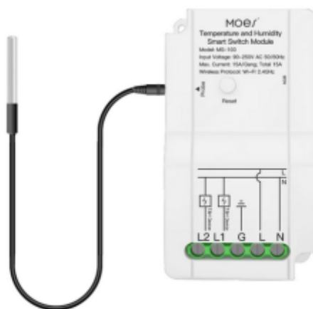
Kit 2: Switch module + Waterproof temperature probe
